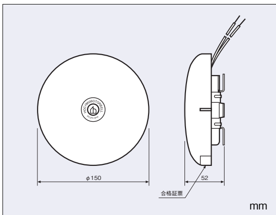
BDP-150I
