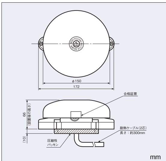
BDO-150JW
